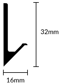
The 32 mm REHAU integrated handle features a visible channel.
